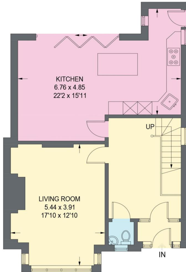
GROUND FLOOR 69.4 SQ M / 747 SQ FT
