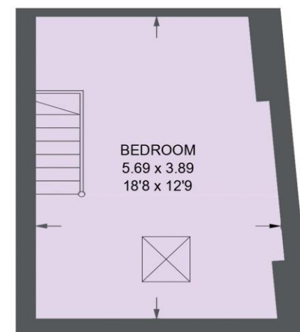
SECOND FLOOR 21.5 SQ M / 231 SQ FT
