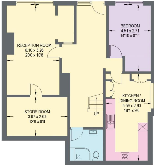
LOWER GROUND FLOOR 84.3 SQ M / 907.9 SQ FT
