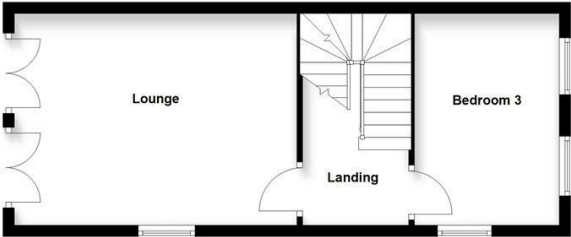
First Floor Approx. 35.8 sq. metres (385.3 sq. feet)
