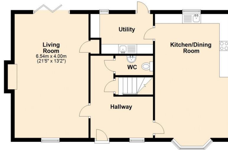
Ground Floor Approx. 76.6 sq. metres (824.6 sq. feet)
