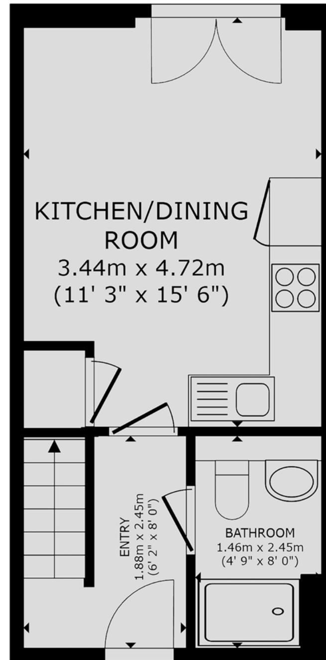
FLOOR 1
