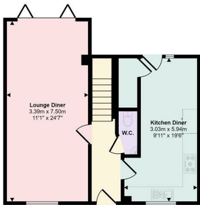
Ground Floor Approx 52 sq m / 565 sq ft
