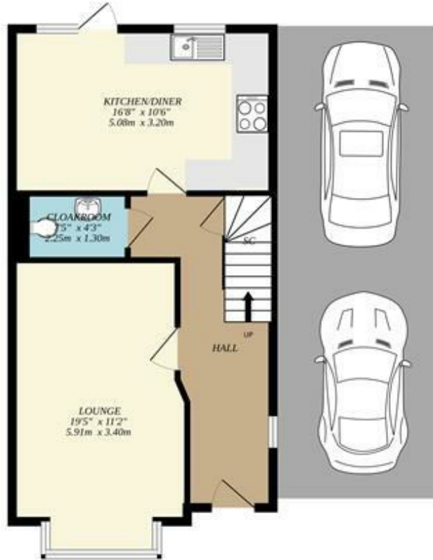
GROUND FLOOR 532 sq.ft. (49.4 sq.m.) approx.
