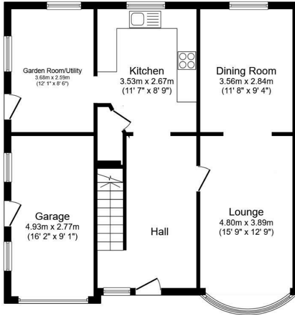
Ground Floor Floor area 75.8 sq.m. (816 sq.ft.)
