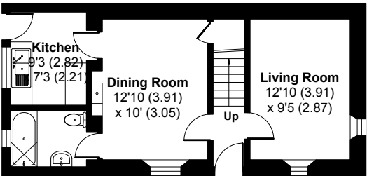
COSAWES BARTON COTTAGE GROUND FLOOR
