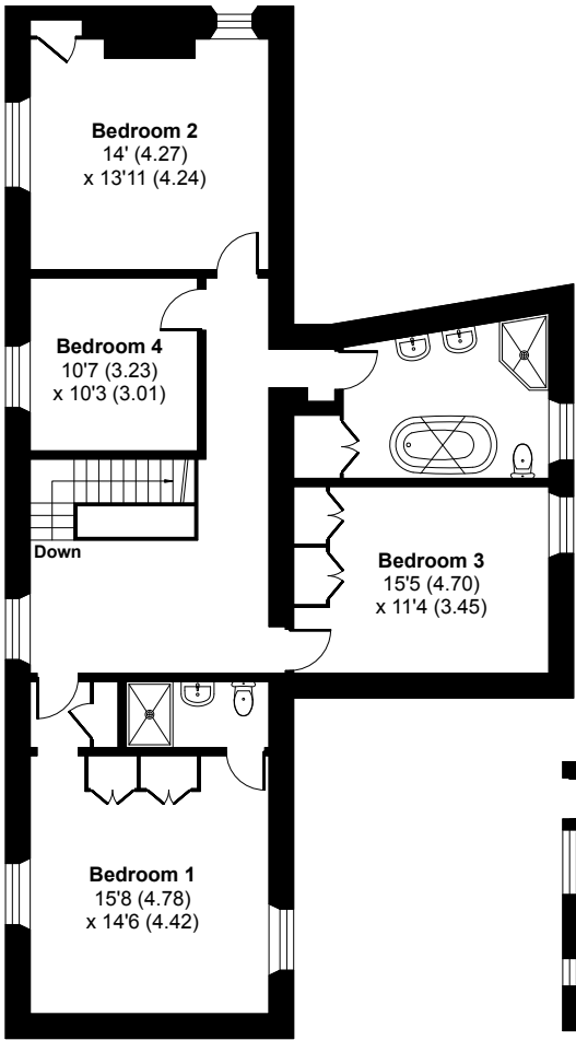
FIRST FLOOR 1
