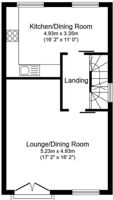
First Floor Floor area 42.6 sq.m. (458 sq.ft.)
