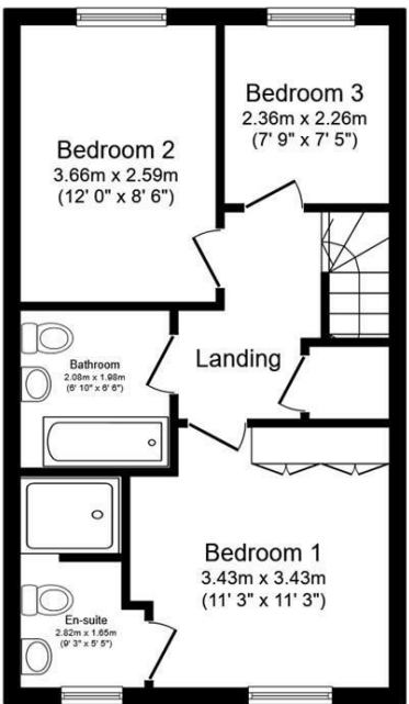
Second Floor Floor area 42.6 sq.m. (458 sq.ft.)
