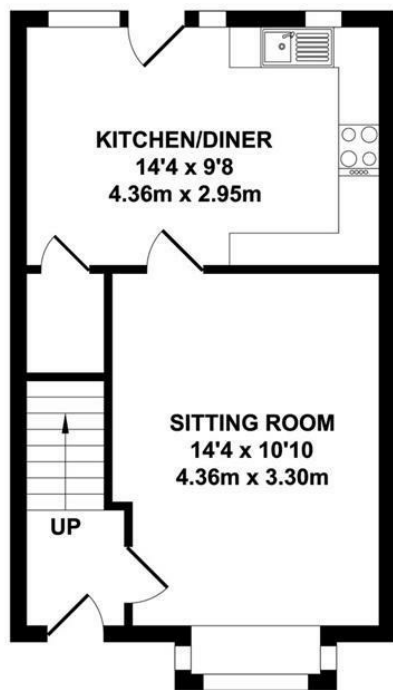
GROUND FLOOR APPROX. FLOOR AREA 358 SQ.FT. (33.26 SQ.M.)
