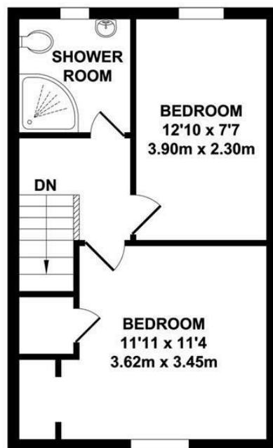
FIRST FLOOR APPROX. FLOOR AREA 348 SQ.FT. (32.30 SQ.M.)
