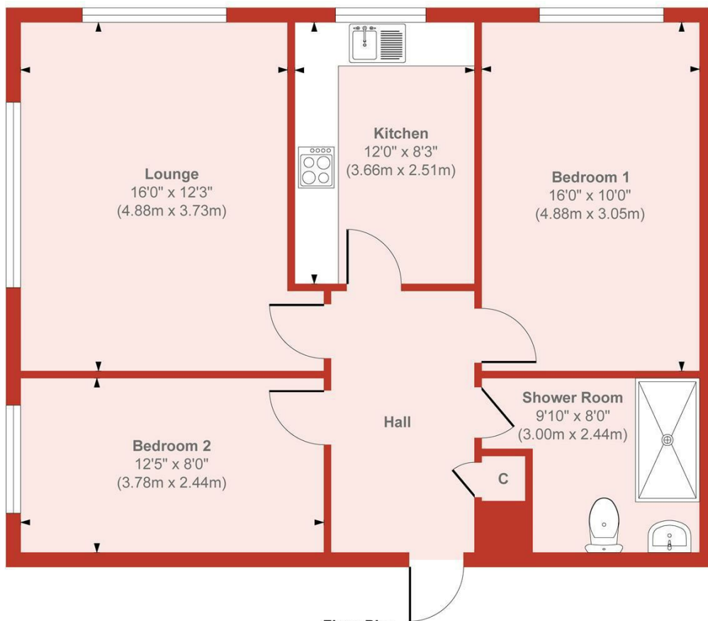
Floor Plan
