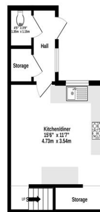
Ground Floor 291 sq. ft. (27.0 sq. m.) approx.
