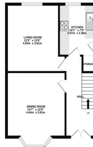
GROUND FLOOR 501 sq.ft. (46.5 sq.m.) approx.
