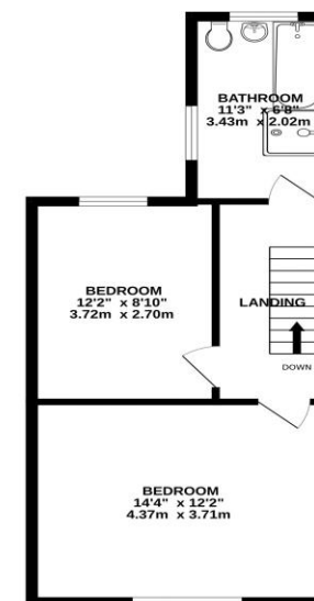
1ST FLOOR 424 sq.ft. (39.4 sq.m.) approx.
