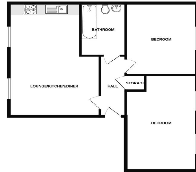
GROUND FLOOR 731 sq.ft. (67.9 sq.m.) approx.
