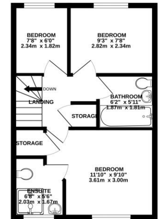
1ST FLOOR 357 sq.ft. (33.2 sq.m.) approx.
