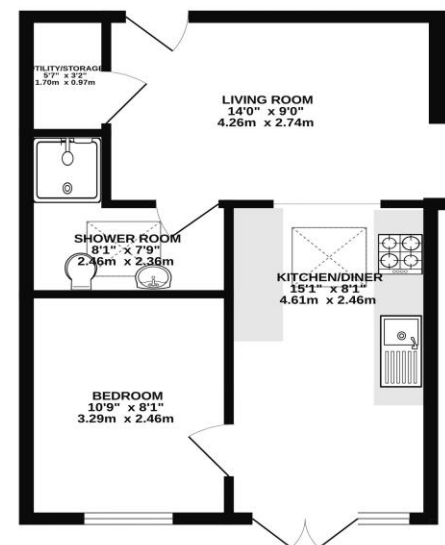
TOTAL FLOOR AREA: 394 sq ft. (36.6 sq.m.) approx. Whilst every attempt has been made to ensure the accuracy of the floorplan contained here, measurements of doors, windows, rooms and any other items are approximate and no responsibility is taken for any error, omission or mis-statement. This plan is for illustrative purposes only and should be used as a guide for any prospective purchaser. The services, systems and appliances shown have not been tested and no guarantee is made as to their operability or efficiency over the years. Made with Metrepro ©2014
