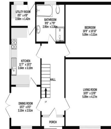
GROUND FLOOR 855 sq.ft. (79.5 sq.m.) approx.
