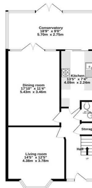
Ground Floor 747 sq. ft. (69.4 sq. m.) approx.
