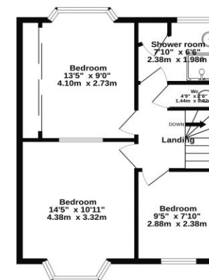
1st Floor 482 sq. ft. (44.8 sq. m.) approx.
