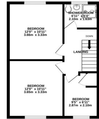
1ST FLOOR 427 sq.ft. (39.7 sq.m.) approx.
