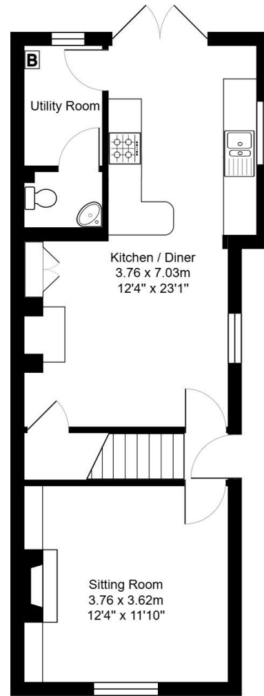
Ground Floor Area: 46.1 m 2 ... 496 ft 2
