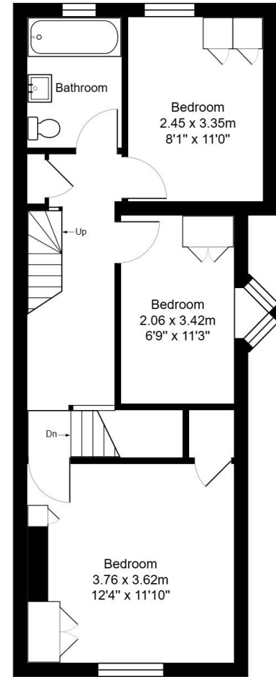
First Floor Area: 46.1 m 2 ... 496 ft 2
