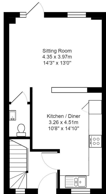
Ground Floor Area: 35.0 m 2 ... 377 ft 2
