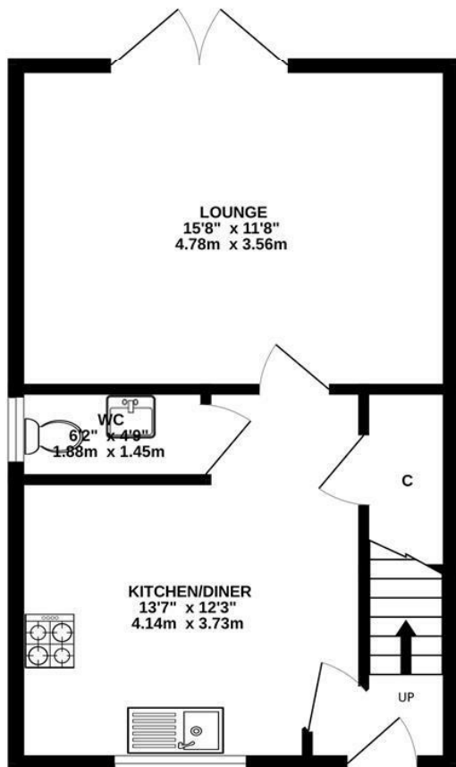
GROUND FLOOR 391 sq.ft. (36.3 sq.m.) approx.
