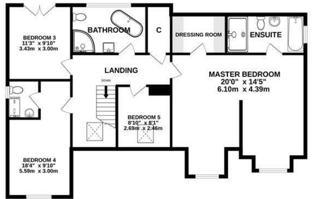
1ST FLOOR 1112 sq.ft. (103.3 sq.m.) approx.
