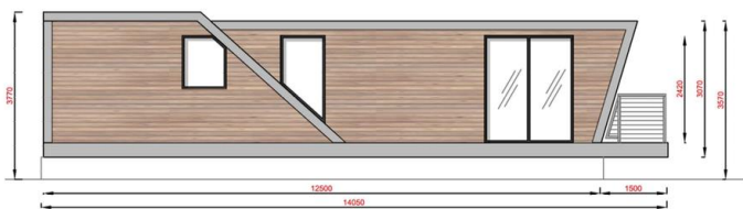
Water Side Elevation SCALE 1:100 @ A3
