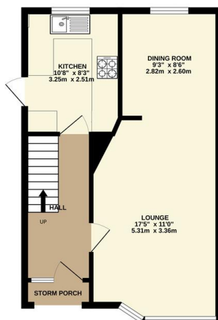
GROUND FLOOR 433 sq.ft. (40.2 sq.m.) approx.
