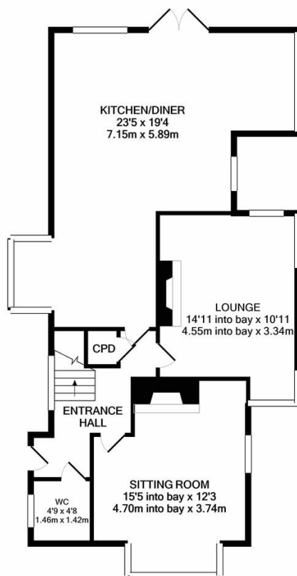
GROUND FLOOR APPROX. FLOOR
