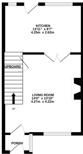
GROUND FLOOR 324 sq.ft. (30.1 sq.m.) approx.
