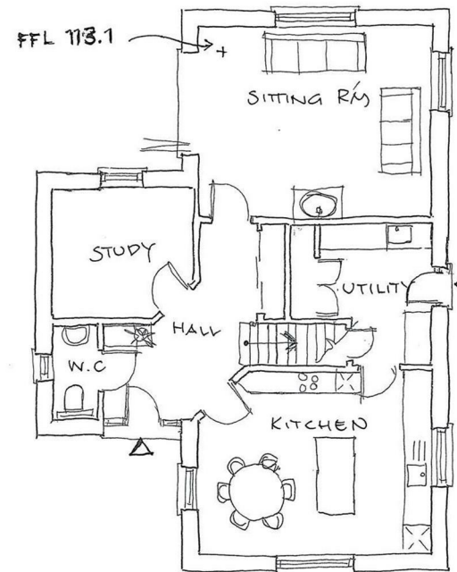
GROUND FLOOR ~ PLOT 2
