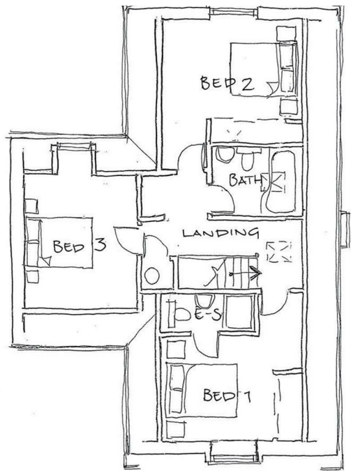
PLOT 2 FIRST FLOOR ~ 1:100
