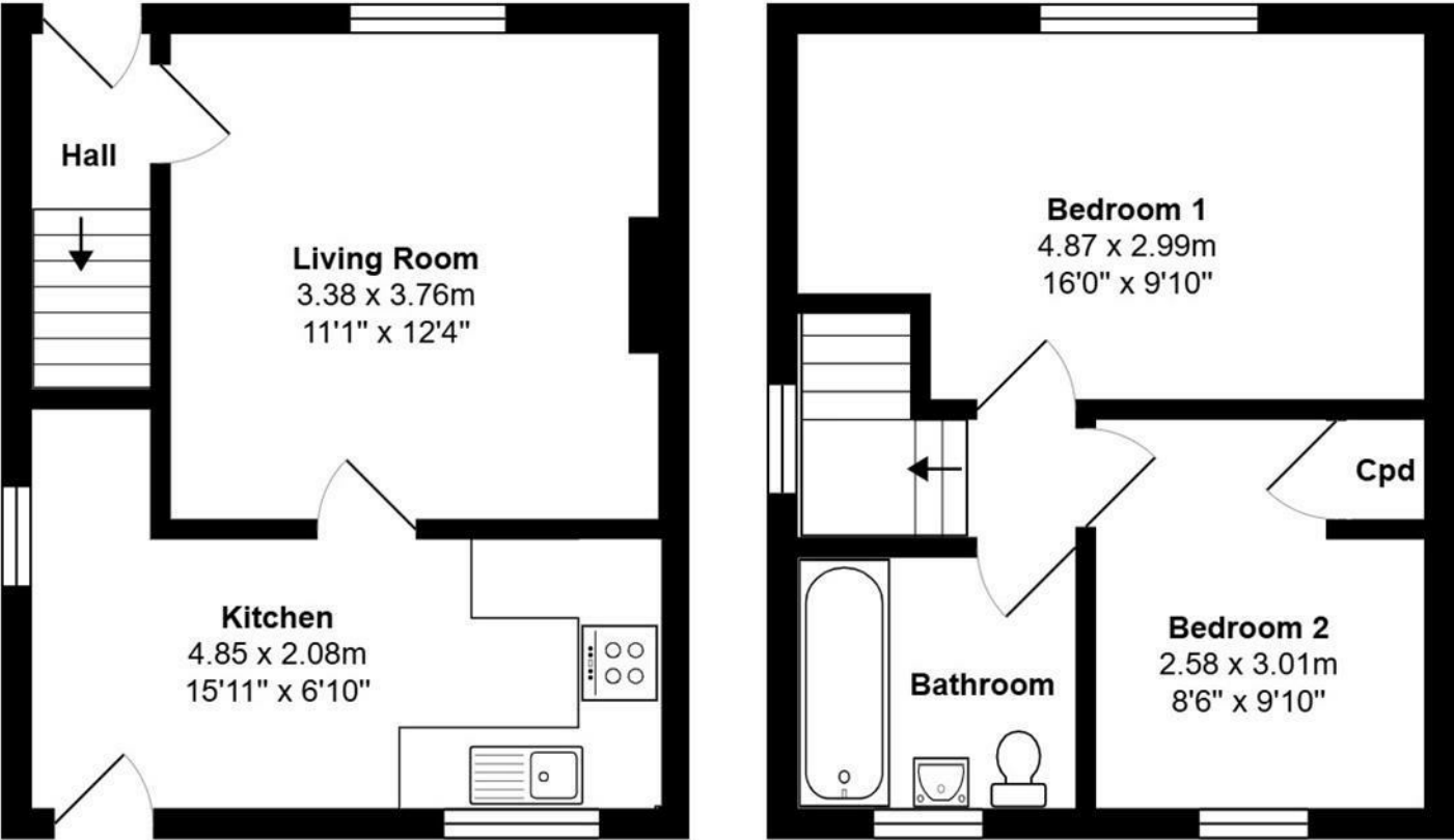
Ground Floor
