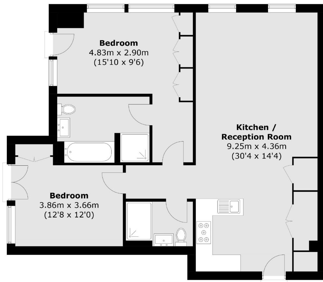
Fourth Floor
