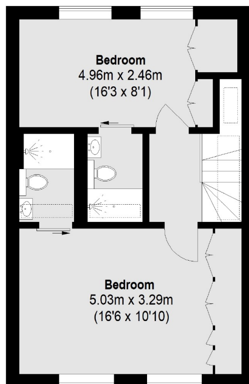
Fourth Floor
