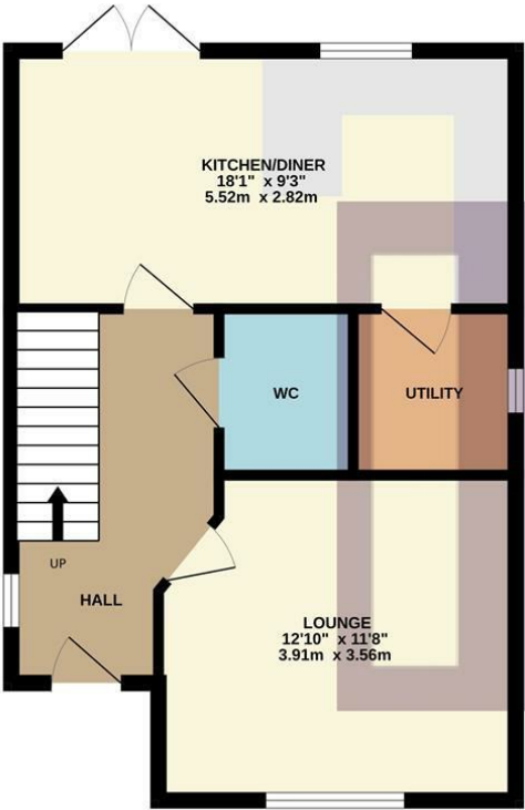
GROUND FLOOR 465 sq.ft. (43.2 sq.m.) approx.
