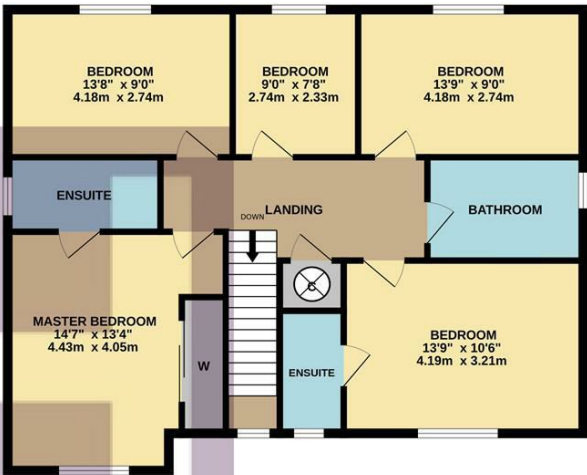
1ST FLOOR 927 sq.ft. (86.1 sq.m.) approx.
