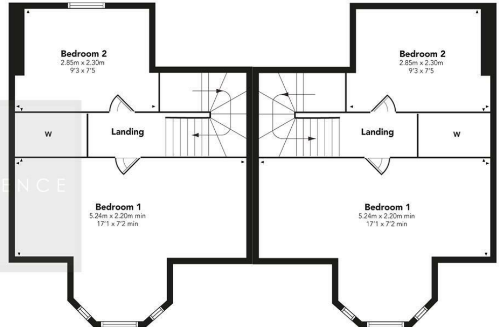
SECOND FLOOR
