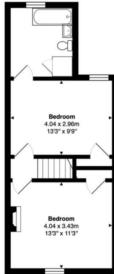
First Floor Area: 37.2 m 2 ... 401 ft 2
