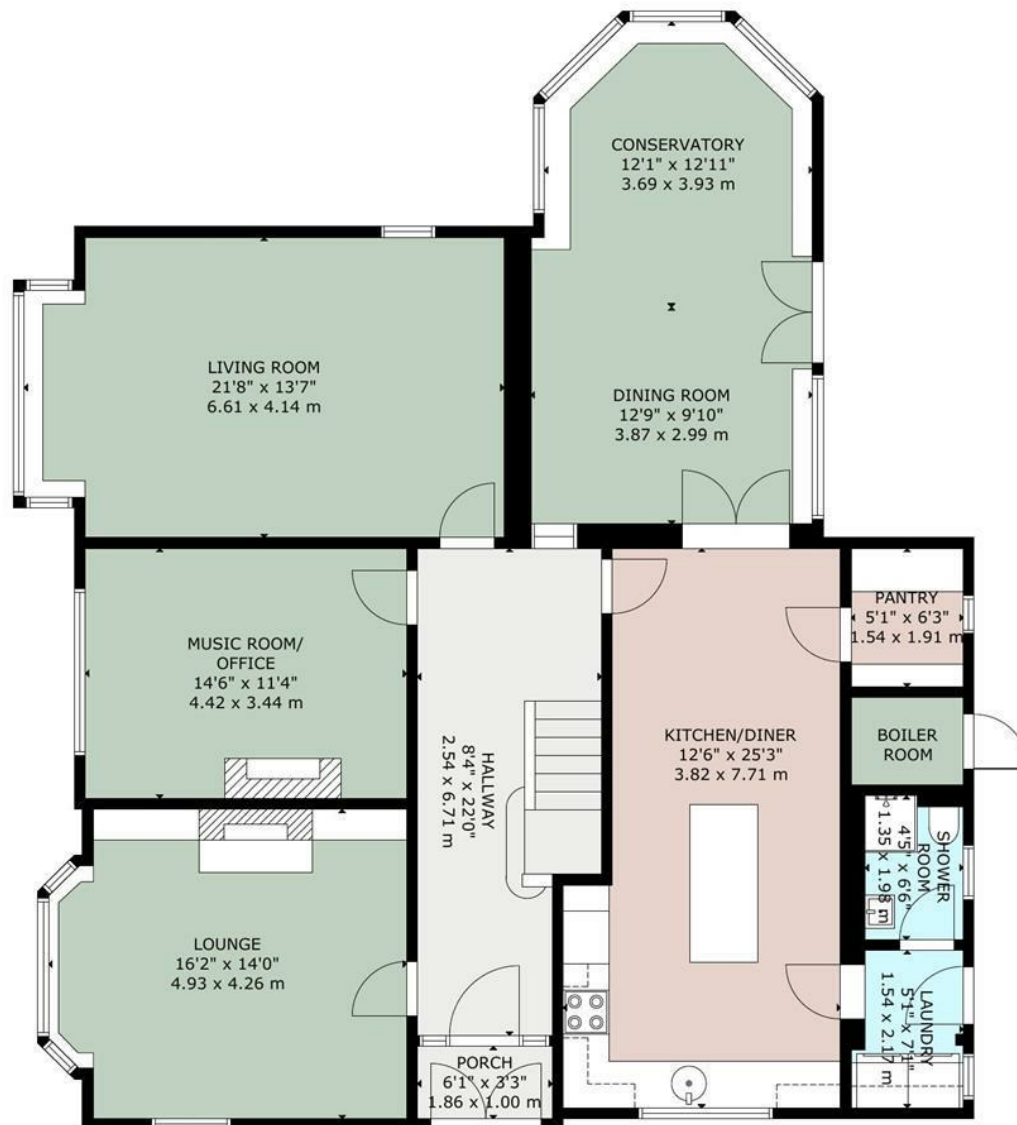
GROUND FLOOR
