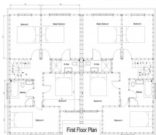
Plot 2 First Floor Plan
