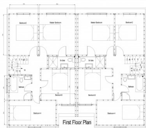
Plot 2 First Floor Plan
