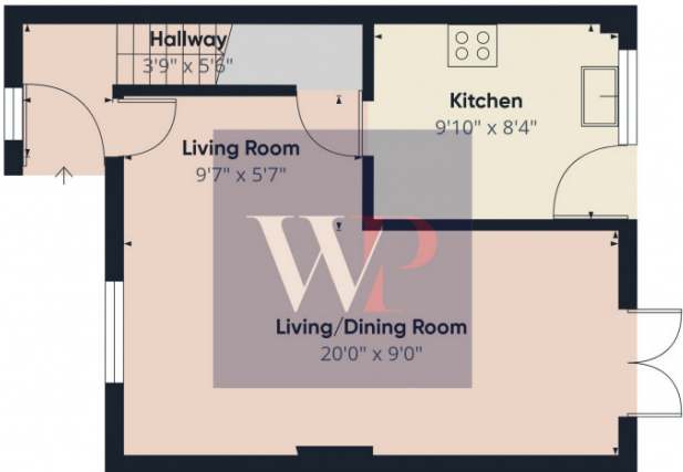
Floor 0 Building 1
