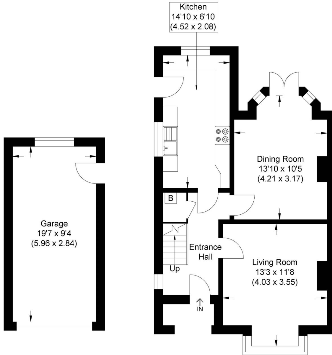
Ground Floor
