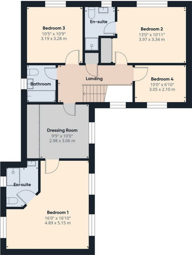
Floor 1
