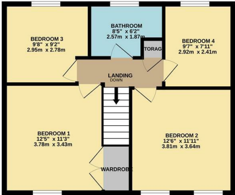
1ST FLOOR 560 sq.ft. (52.1 sq.m.) approx.
