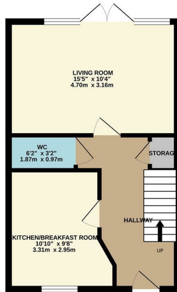
GROUND FLOOR 376 sq.ft. (34.9 sq.m.) approx.
