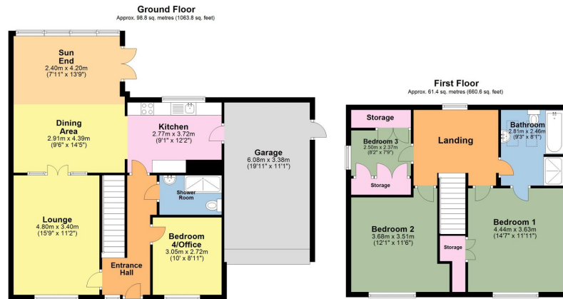
Total area: approx. 160.2 sq. metres (1724.4 sq. feet) These are approximate dimensions. Plan produced using PlanIt.
