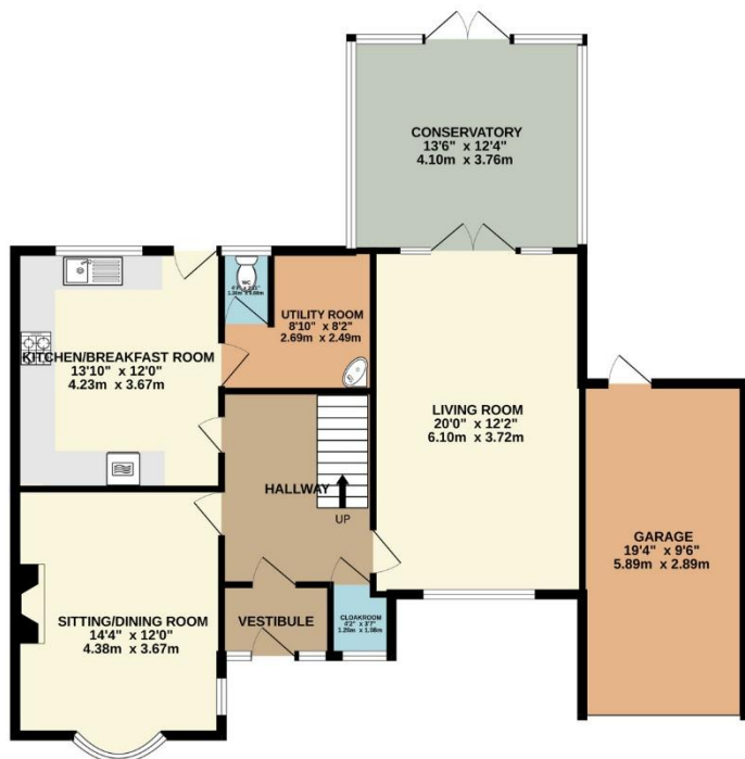
GROUND FLOOR 1143 sq.ft. (106.2 sq.m.) approx.
