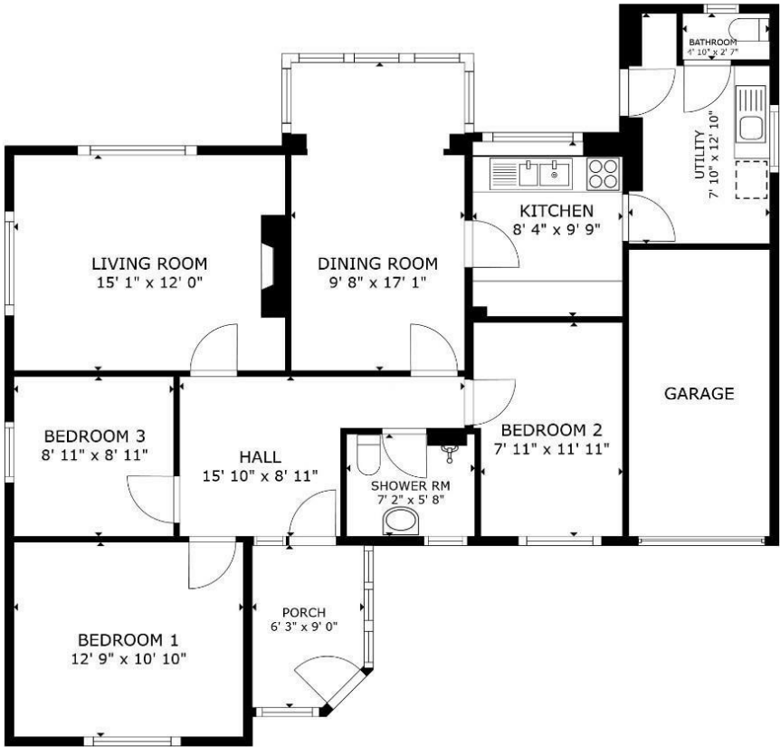
FLOOR PLAN
