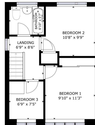
FIRST FLOOR PLAN FLOOR 2: 1047 SQ. FT. (97 SQ. METERS) TOTAL AREA: 2094 SQ. FT. (194 SQ. METERS)
